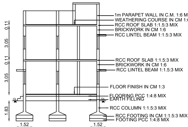
CROSS SECTION ON XY
