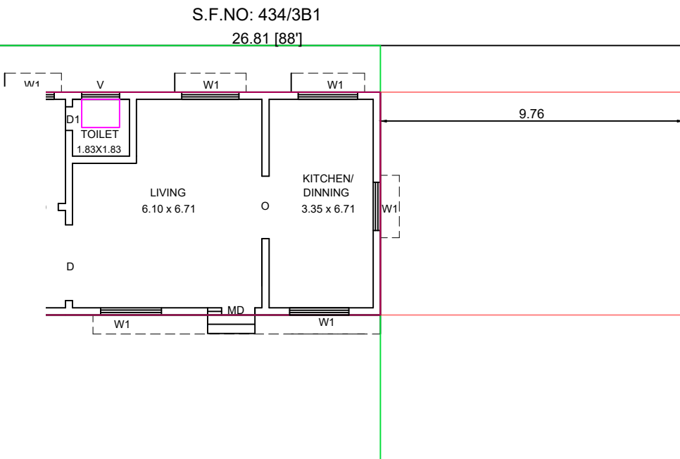
GROUND FLOOR & SITE PLAN SITE PLAN (SCALE 1:100)
