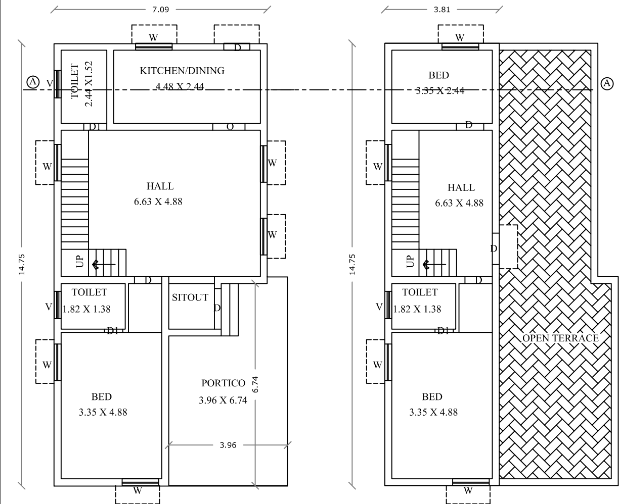
PRO. FIRST Floor Plan
