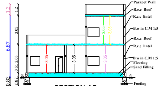
SECTION AB
