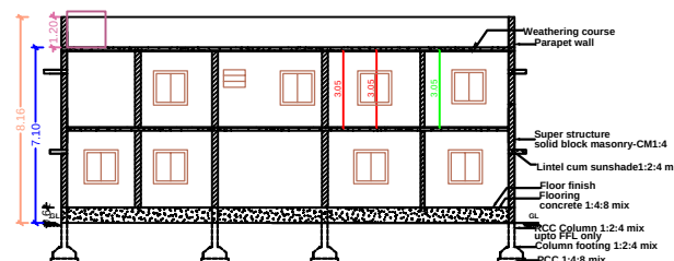
SECTION ELEVATION
