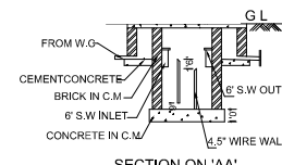
SECTION ON A'A'
