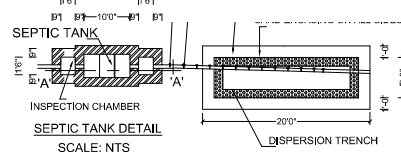
SEPTIC TANK DETAIL SCALE: NTS
