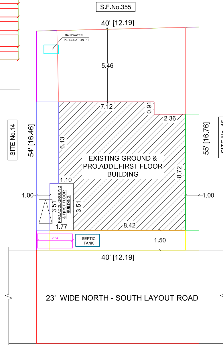
SITE PLAN
