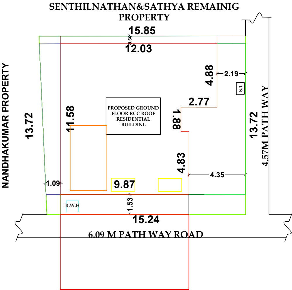
SITE PLAN
