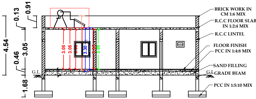
SECTION
