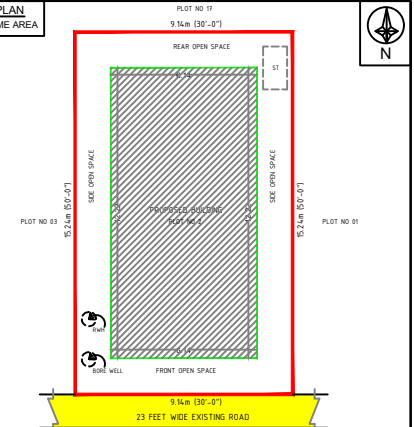
PLAN SHOWING THE PROPOSED CONSTRUCTION OF A RESIDENTIAL BUILDING IN S.NO.45/3B, PLOT NO:2, DEEPAM GARDEN-II, KURUDAMPALAYAM VILLAGE & PANCHAYAT, COIMBATORE NORTH TALUK, COIMBATORE DISTRICT SCALE : 1"=100'
