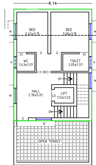
PRO.FIRST FLOOR PLAN
