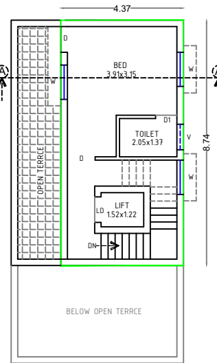
PRO.SECOND FLOOR PLAN
