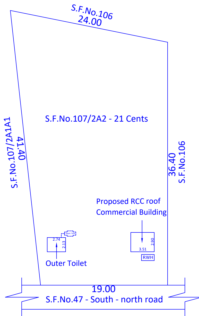
SITE PLAN
