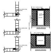
EARTHQUAKE SAFE DESIGN (NOT TO SCALE)
