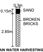
DETAIL PERCOLATION PIT (NTS)
