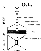
FOUNDATION DETAILS (NOT TO SCALE)
