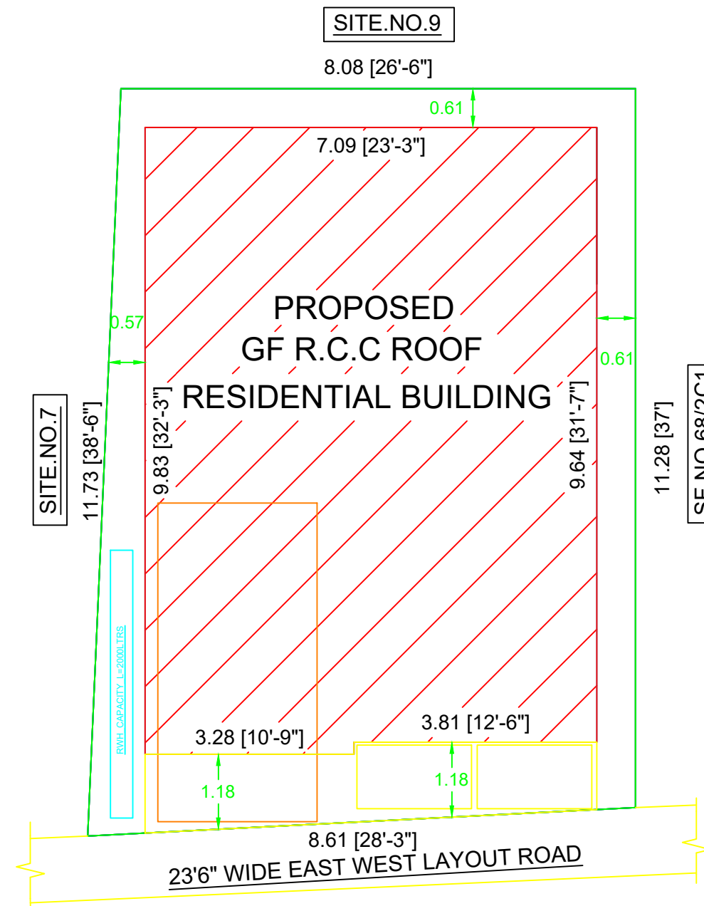
SITE PLAN
