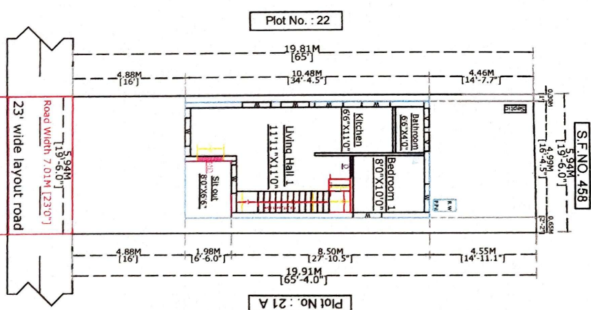
Site cum Pro. Ground Floor Plan
