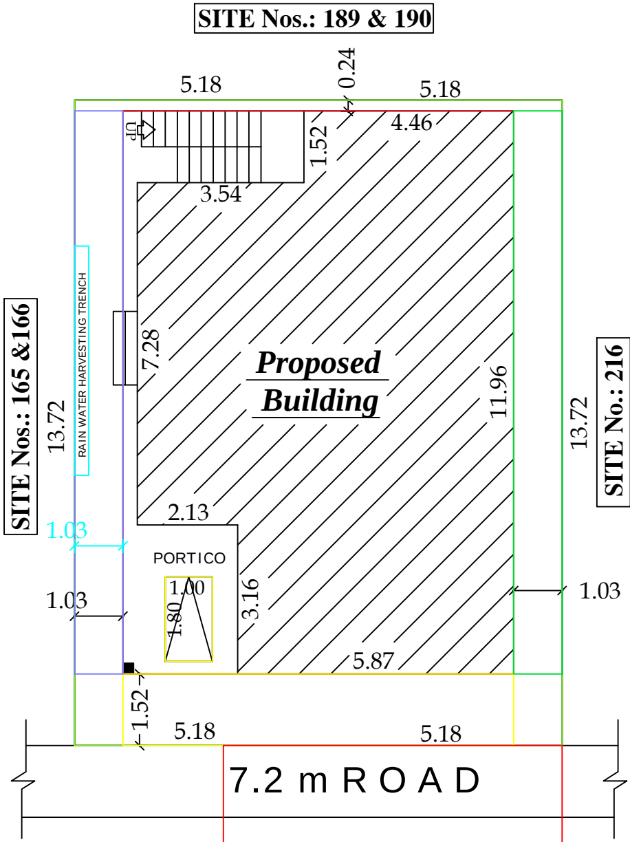
SITE PLAN
