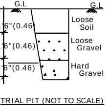
TRIAL PIT (NOT TO SCALE)
