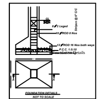
FOUNDATION SECTION (NOT TO SCALE)
