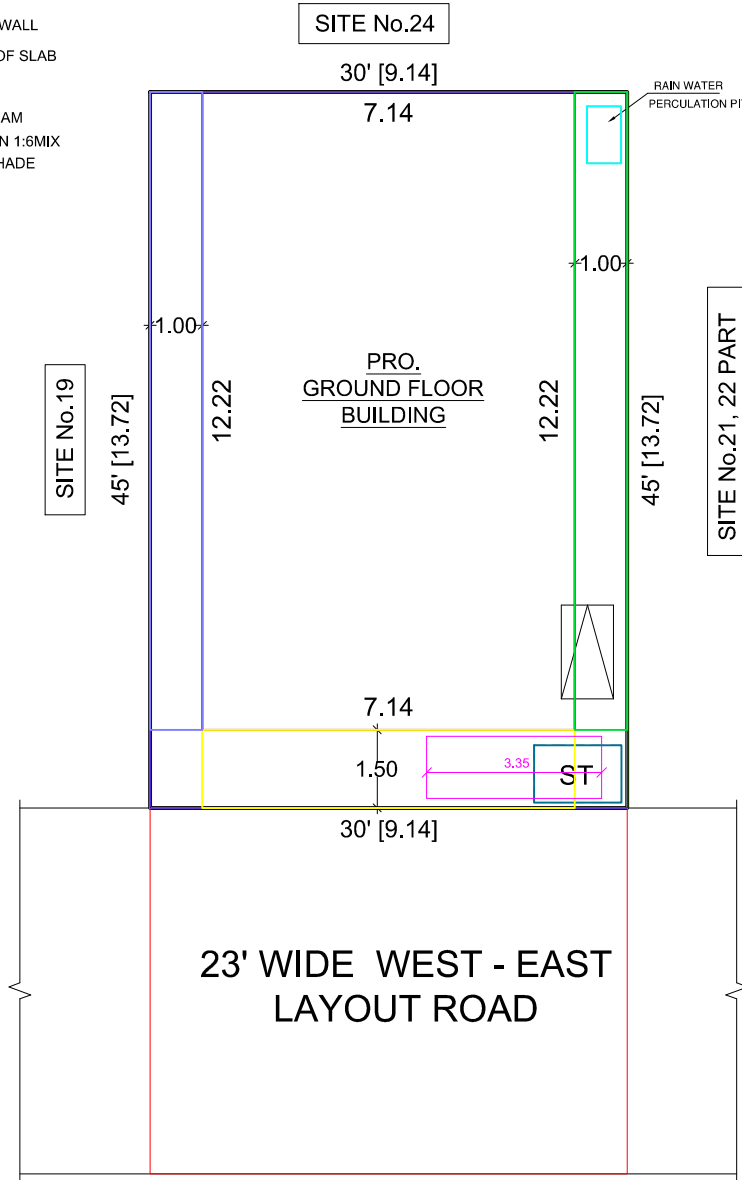
SITE PLAN
