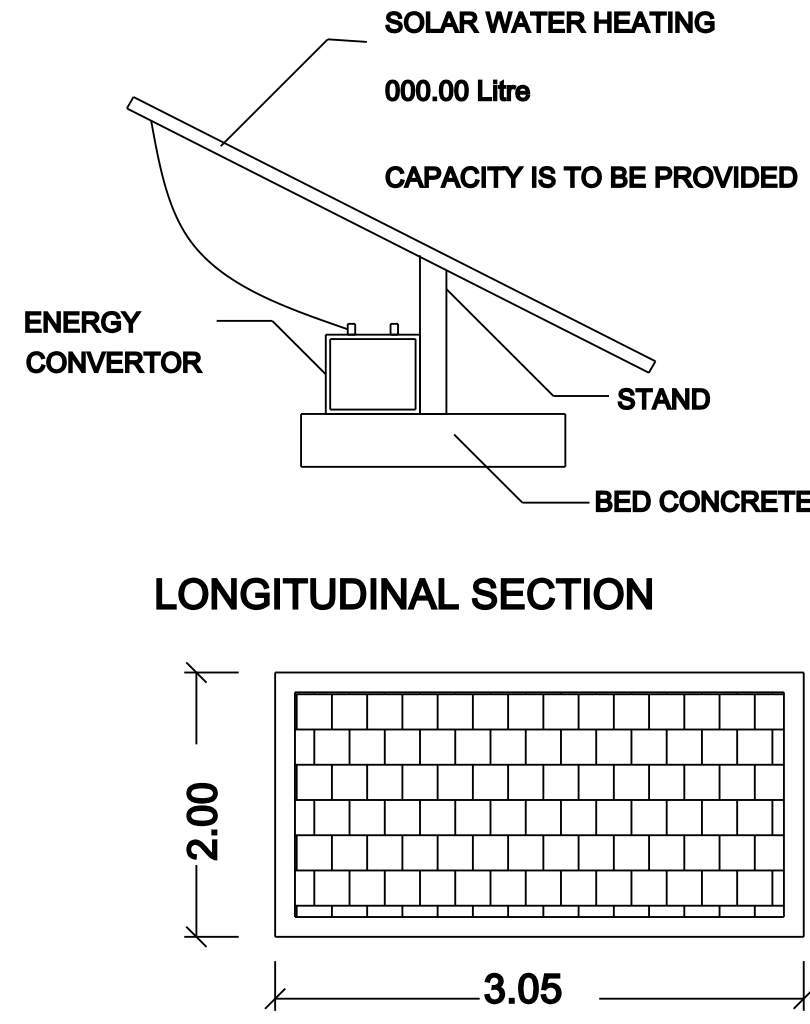
SOLAR SYSTEM
