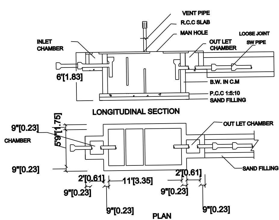
SEPTIC TANK:
