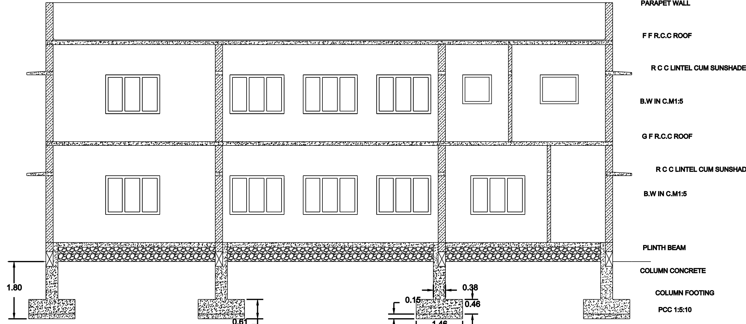
SECTION AB
