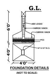
EARTHQUAKE SAFE DESIGN (NOT TO SCALE)
