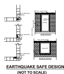
SEISMIC REINFORCEMENT DETAILS (NOT TO SCALE)
