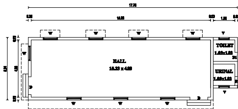
PLAN-3
