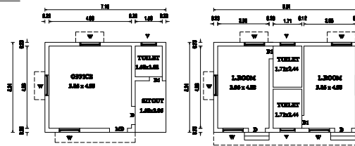
PLAN-1
