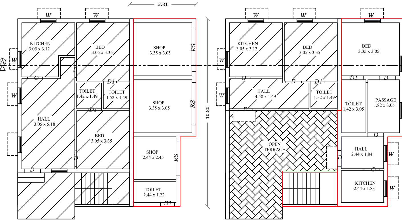
AN EXIS. & PRO. GROUND FLOOR PLAN
