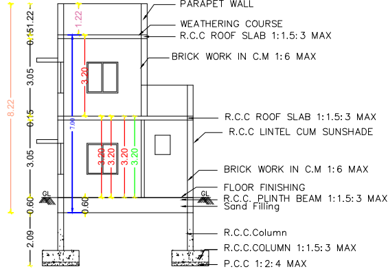
SECTION AT AA
