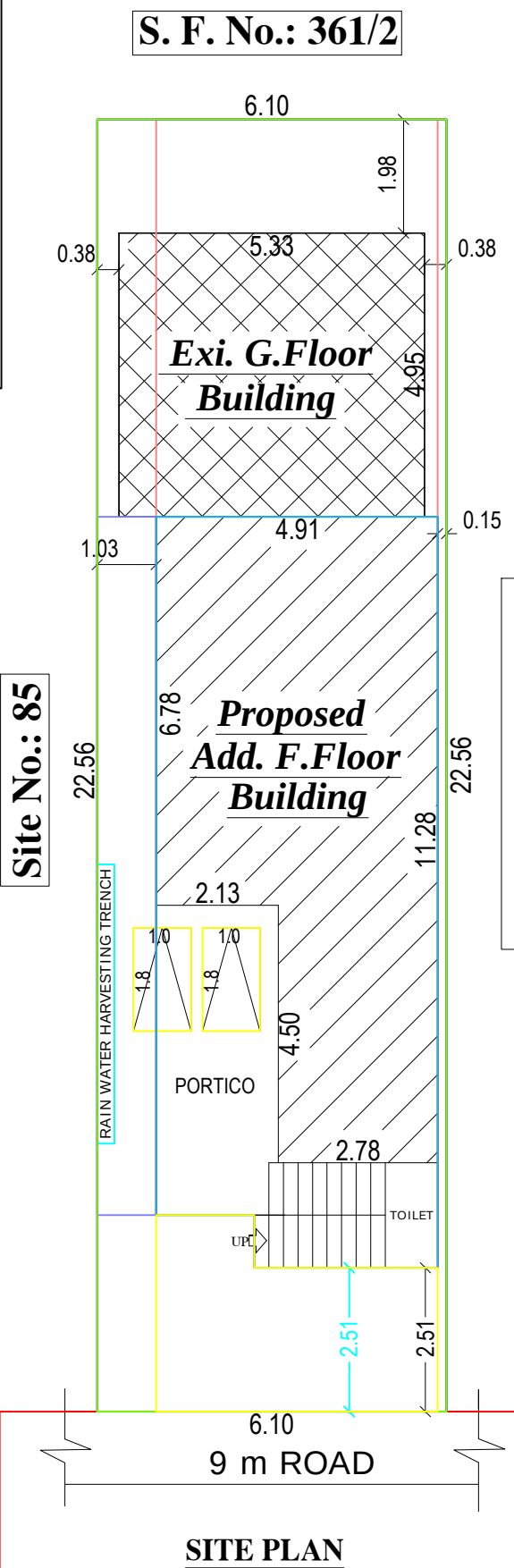
SITE PLAN
