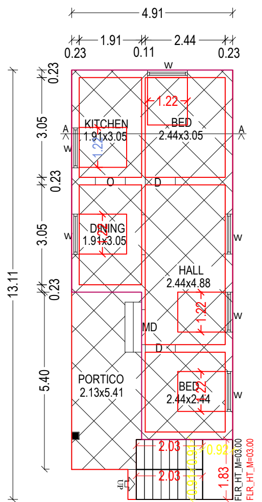
EXI. GROUND FLOOR PLAN
