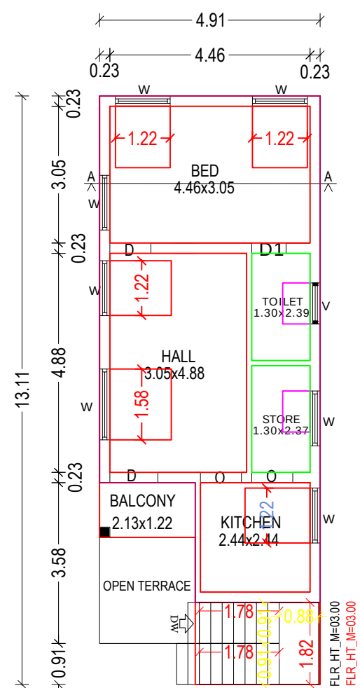
PRO. ADD. FIRST FLOOR PLAN
