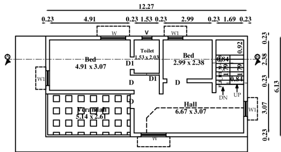
Pro.First Floor Plan
