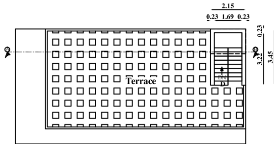
Pro.Head Room Plan
