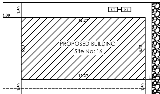
Site Plan
