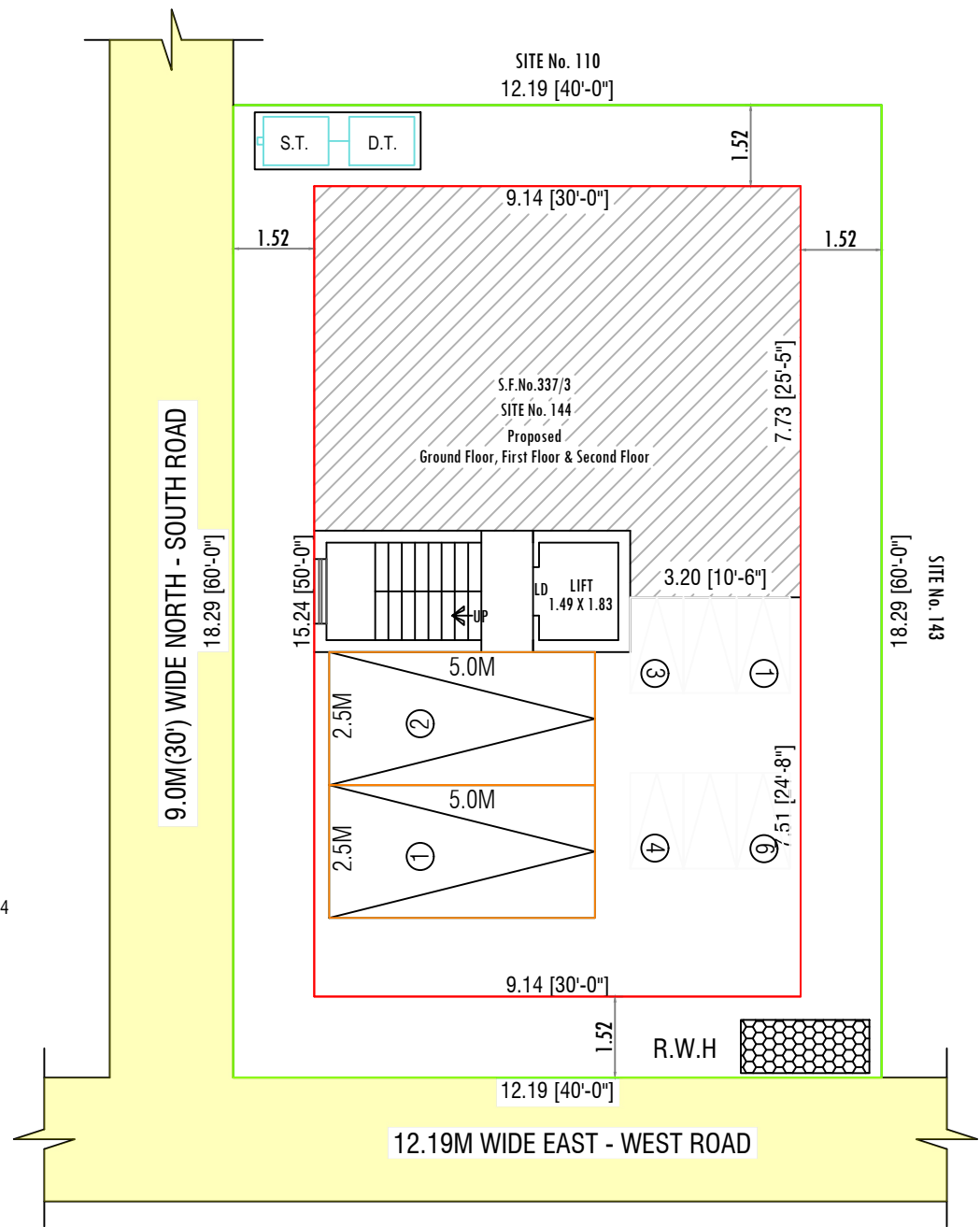
SITE PLAN
