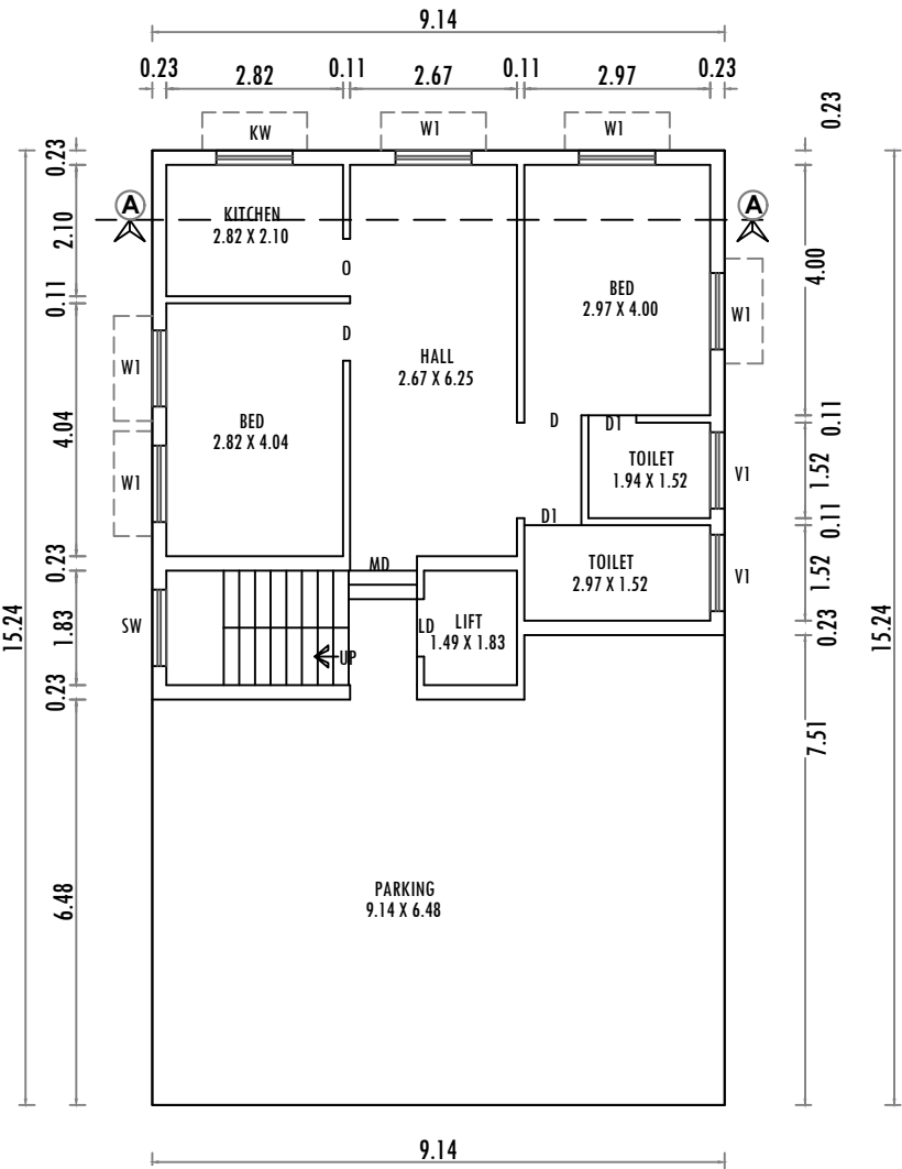
GR PLAN
