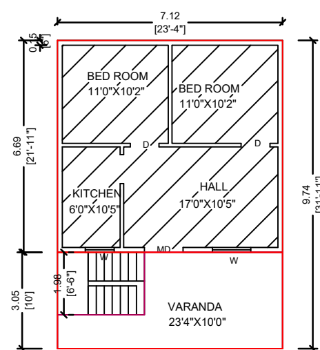
Ex.building & addtional G.F Building
