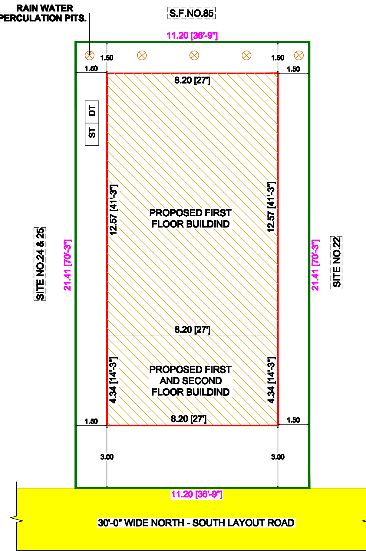
SITE PLAN
