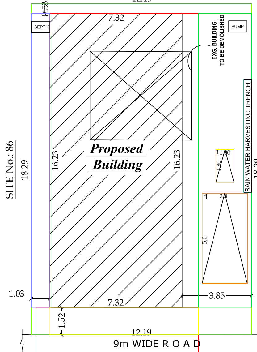
SITE PLAN
