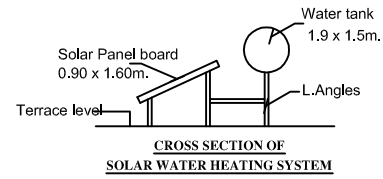
CROSS SECTION OF SOLAR WATER HEATING SYSTEM
