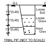
TRIAL PIT (NOT TO SCALE)
