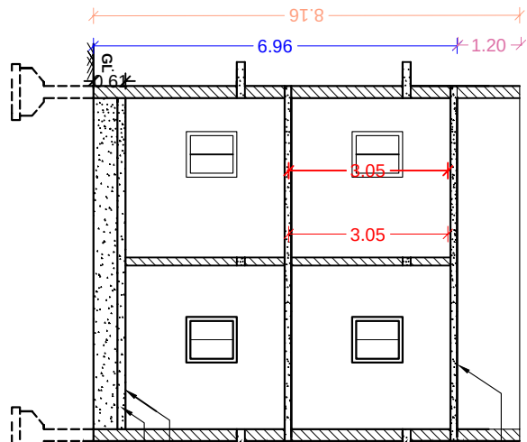
SECTION ELEVATION
