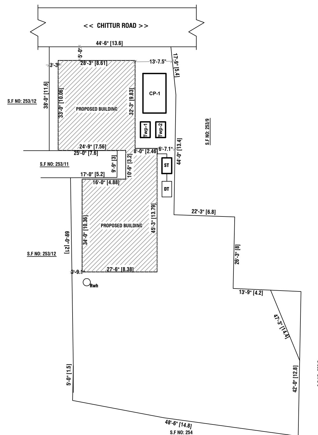
SITE PLAN
