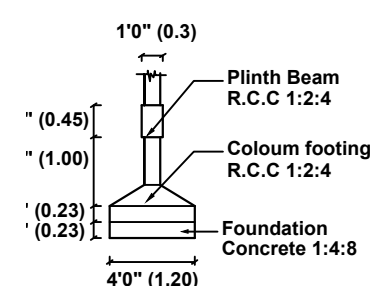
Footing details
