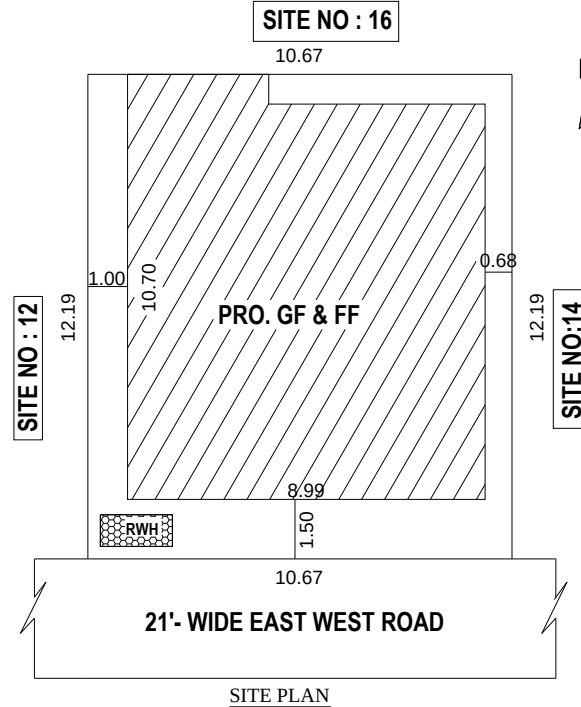
SITE PLAN
