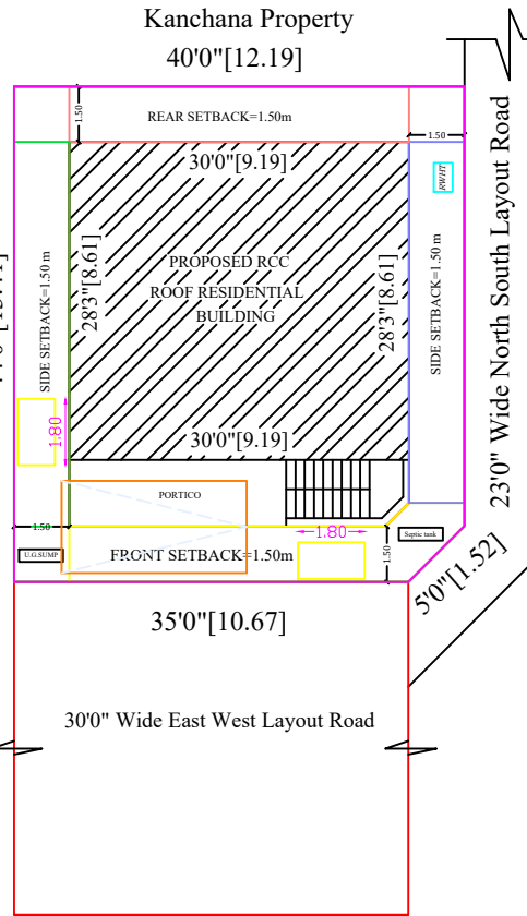
SITE PLAN
