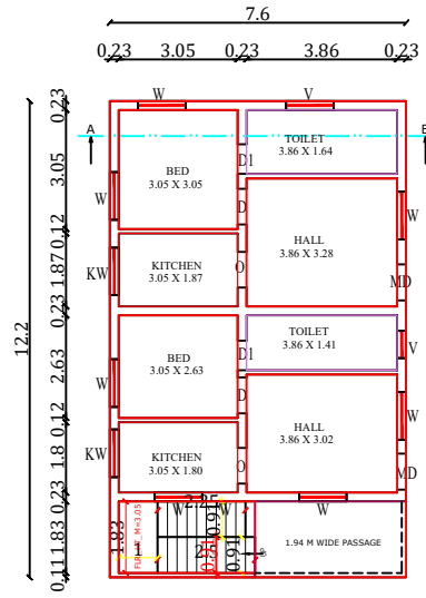
PRO.G.FLOOR PLAN
