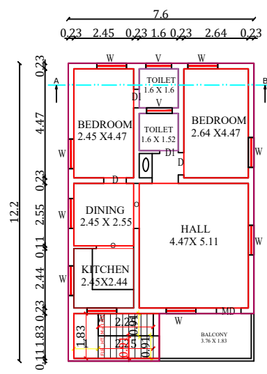
PRO.F.FLOOR PLAN
