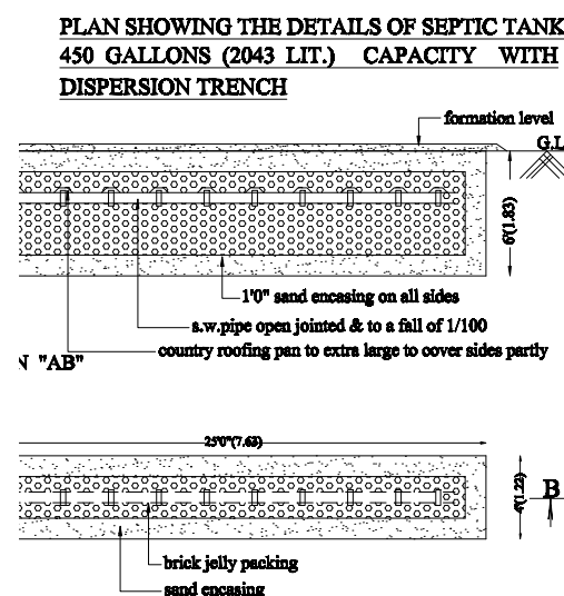
DISPERSION TRENCH
