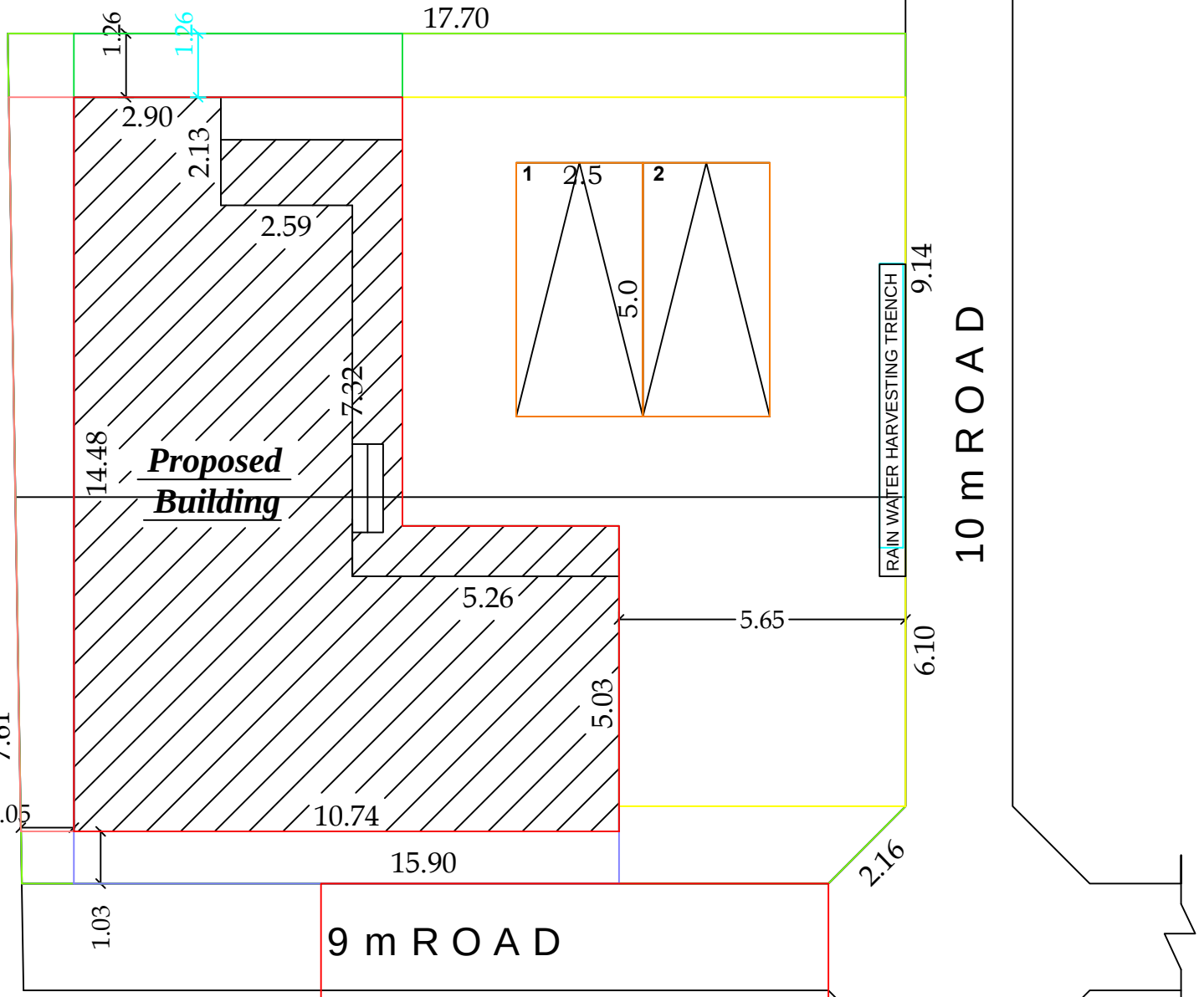
SITE PLAN
