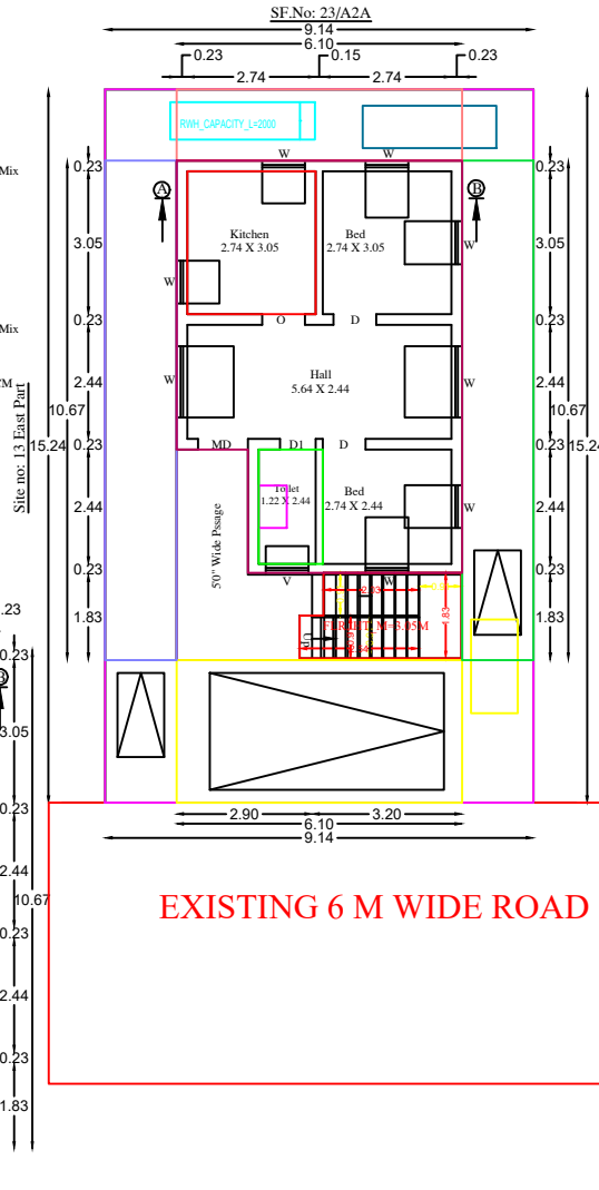
SITE PLAN & EXISTING GROUND FLOOR PLAN
