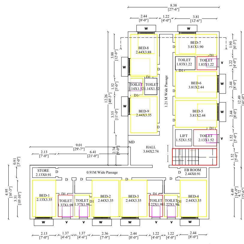
GROUND FLOOR PLAN(LODGE)
