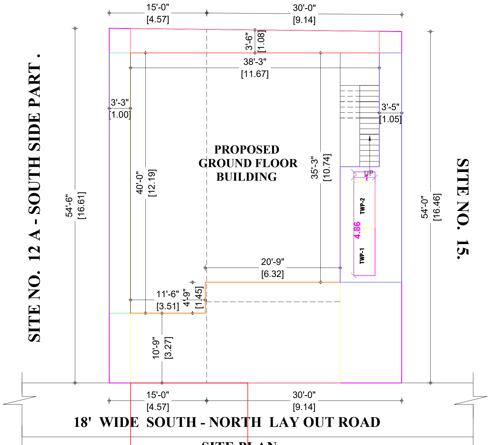
SITE PLAN
