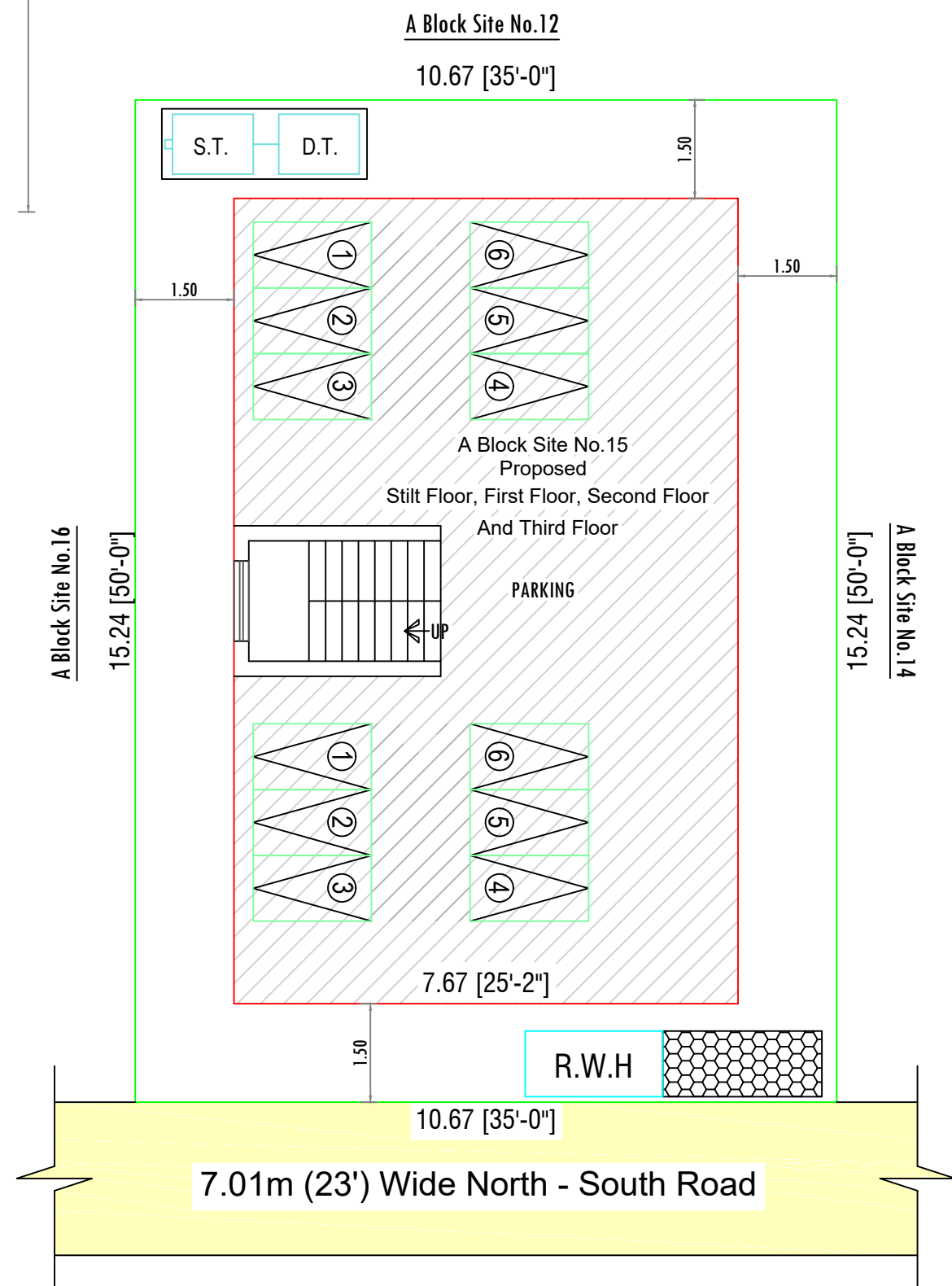
SITE PLAN
