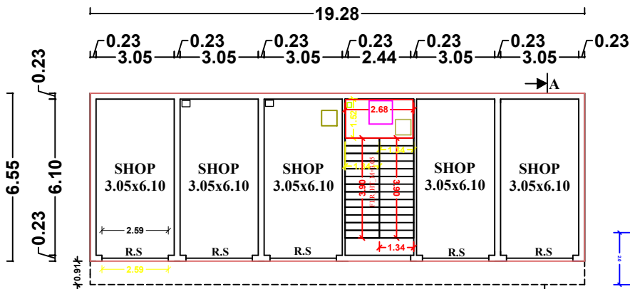
EXISTING GROUND FLOOR
