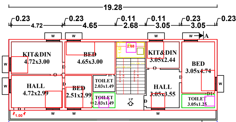
PROPOSED FIRST FLOOR
