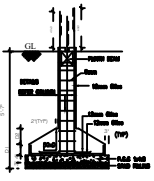
FOUNDATION DETAILS SCALE : 1:50.
