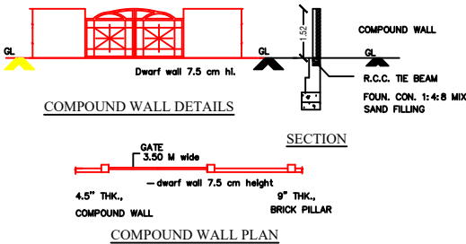
COMPOUND WALL PLAN
