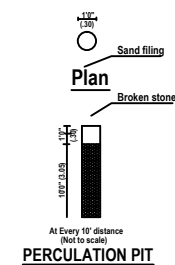
(Not to scale) PERCULATION PIT
