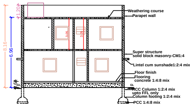
SECTION ELEVATION
