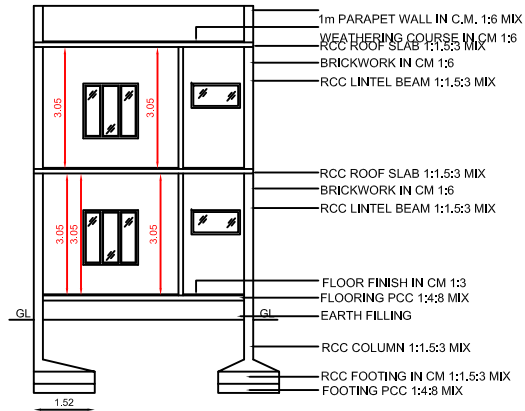
CROSS SECTION ON XY
