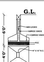
FOUNDATION DETAILS (NOT TO SCALE)
