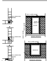
EARTHQUAKE SAFE DESIGN (NOT TO SCALE)
