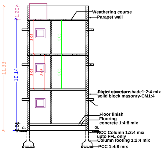
SECTION ELEVATION
