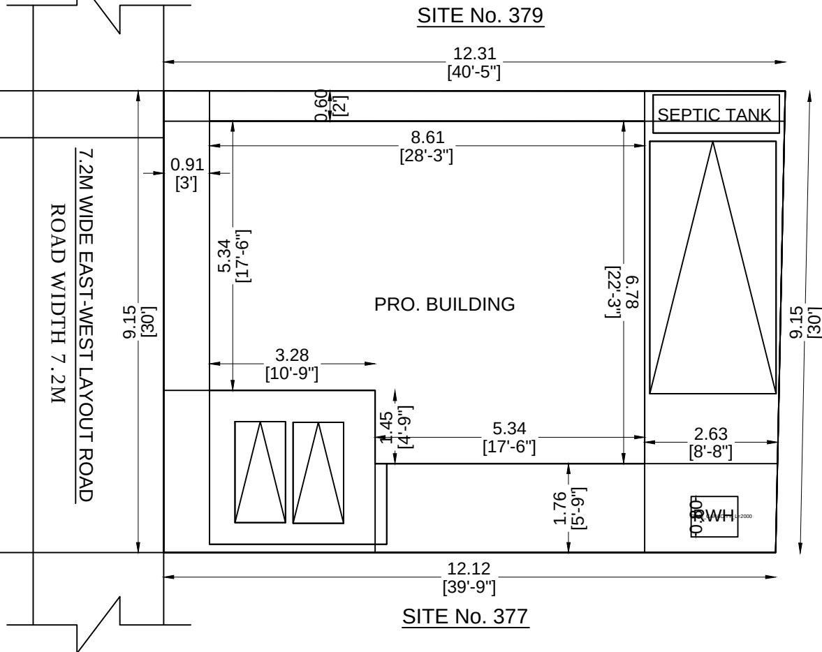
SITE PLAN
