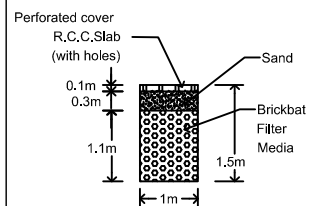
RAIN WATER HARVESTING RECHARGE TRENCH SECTION
