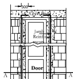
Sectional Elevation Of Door
