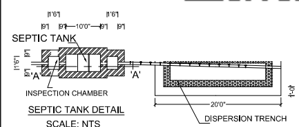
SEPTIC TANK SCALE: NTS
