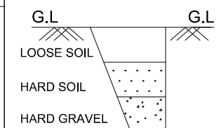
TRIAL PIT SCALE: NTS
