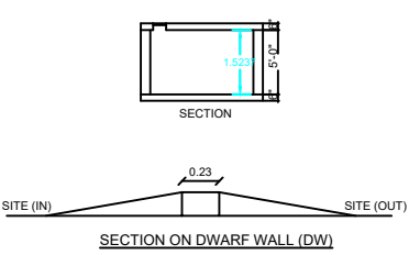
SECTION ON DWARF WALL (DW)
