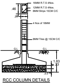
RCC COLUMN DETAILS
