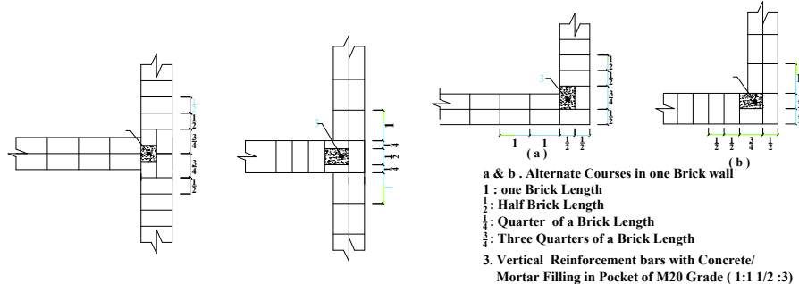
Figure - 3 : Typical Details of Providing Vertical Steel bars in Brick Masonry.
