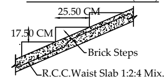
STAIRCASE DETAILS (NTS)
