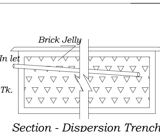
Section - Dispersion Trench
