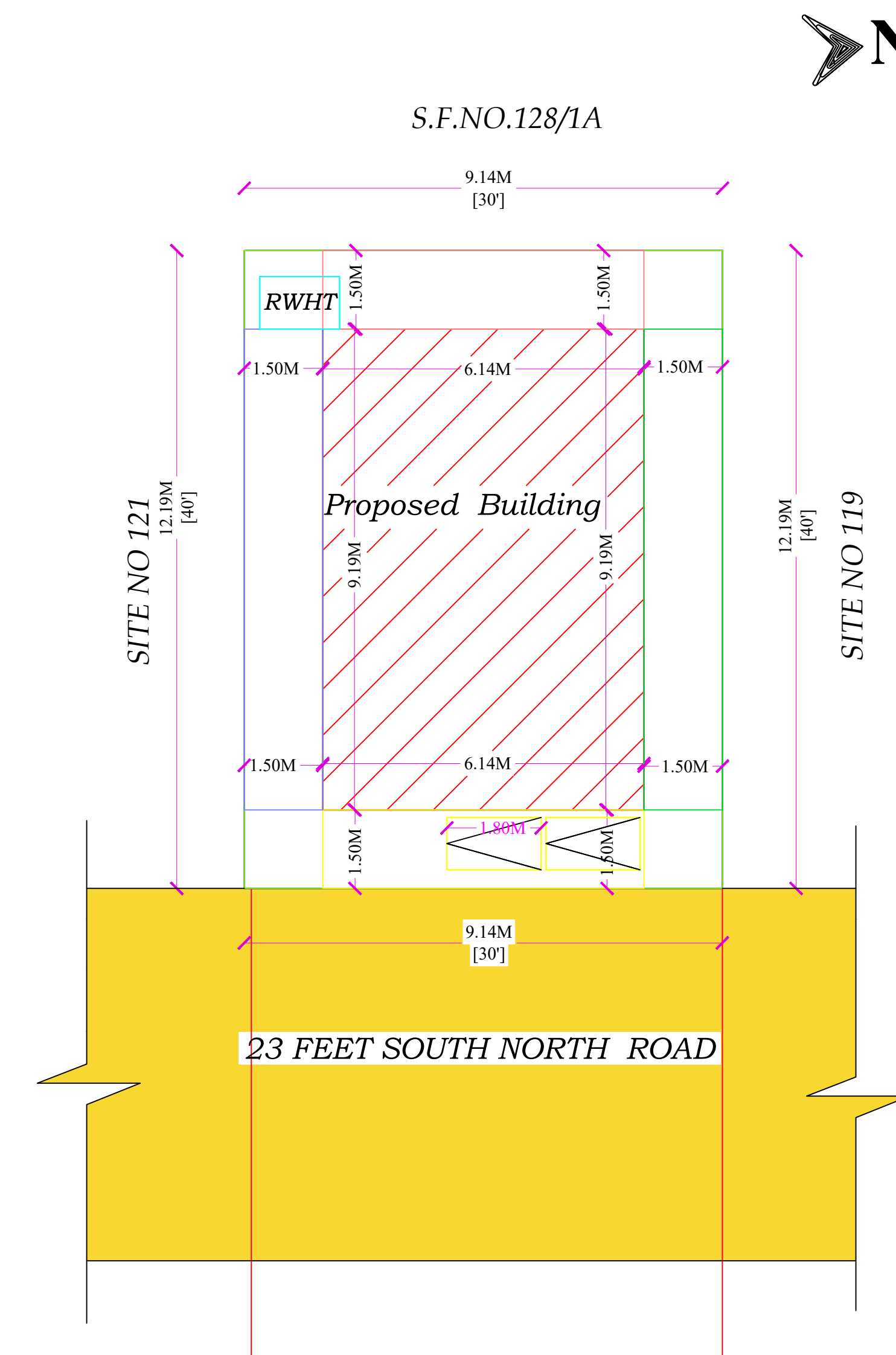
Site Plan (Scale 1":8'0") SITE PLAN
