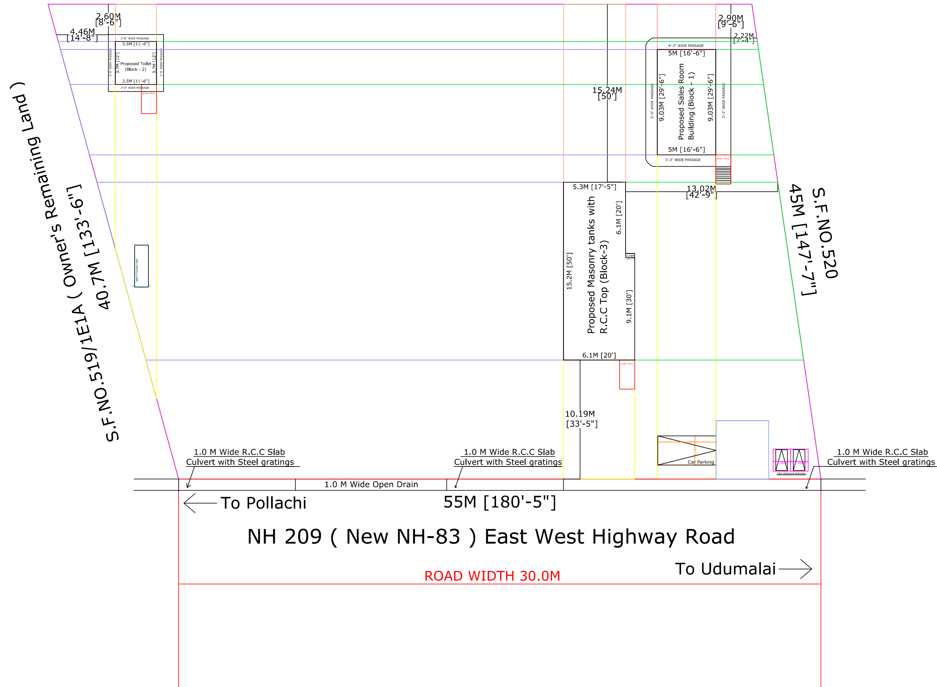
SITE PLAN
