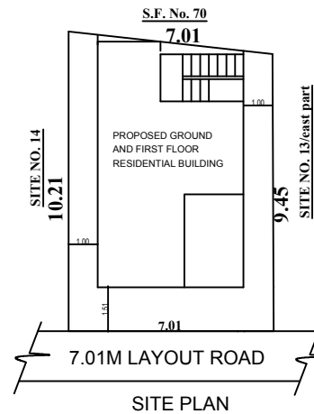
SITE PLAN
